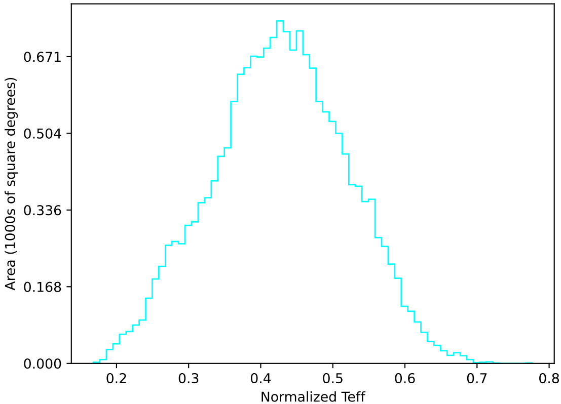
too_ignore_10_1v3.4_10yrs WFD u band: Normalized Teff
