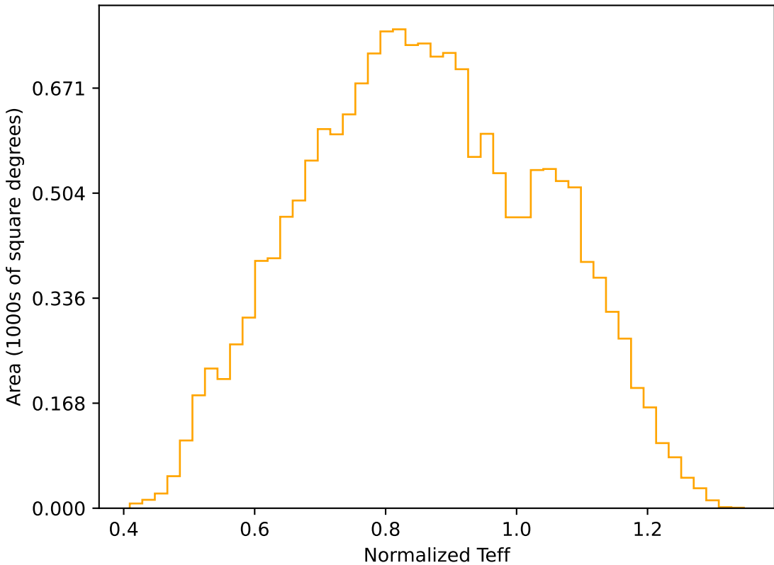
too_ignore_10_1v3.4_10yrs WFD r band: Normalized Teff
