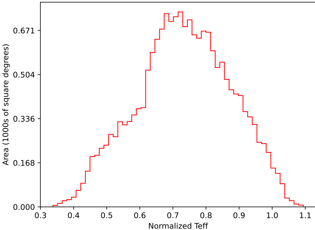
too_ignore_10_1v3.4_10yrs WFD i band: Normalized Teff
