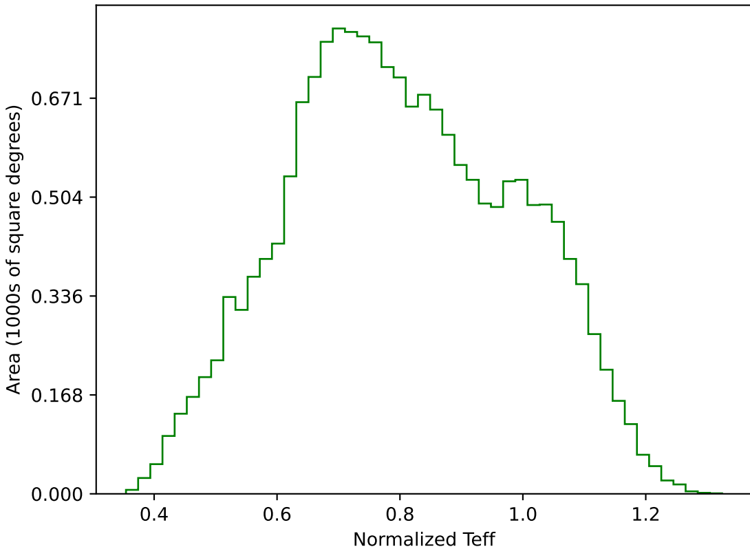
too_ignore_10_1v3.4_10yrs WFD g band: Normalized Teff
