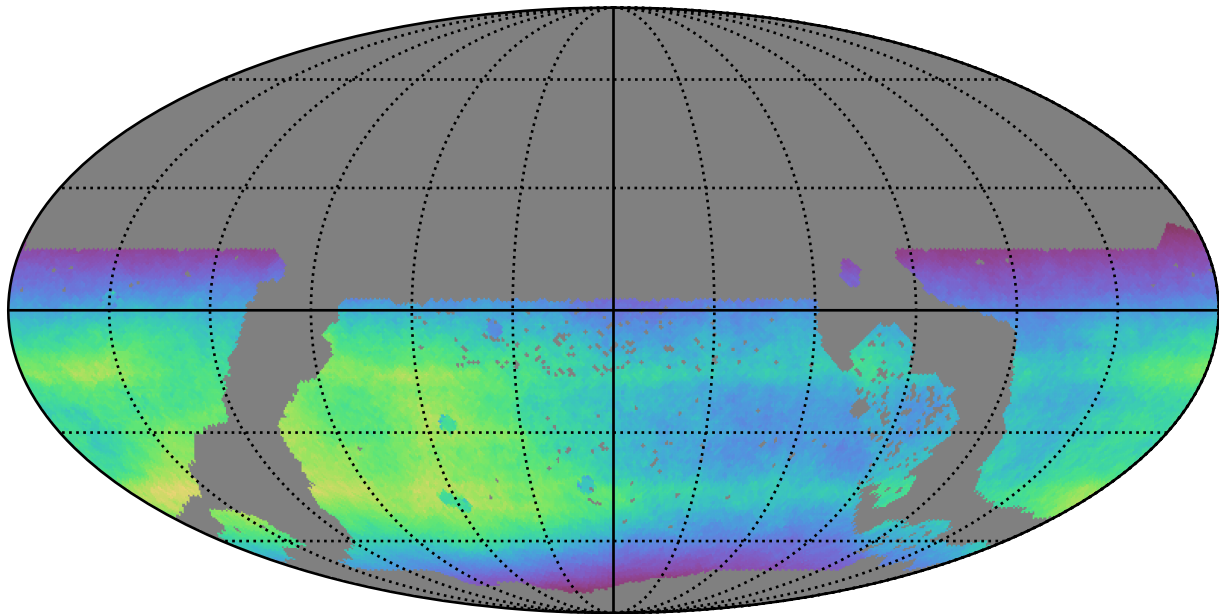
too_ignore_10_1v3.4_10yrs WFD all bands: Normalized Teff
