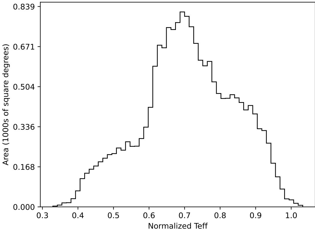
too_ignore_10_1v3.4_10yrs WFD all bands: Normalized Teff
