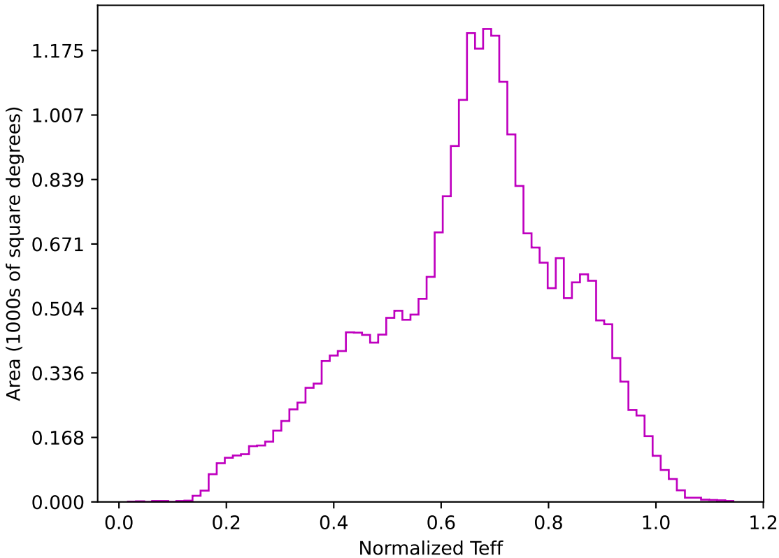
too_ignore_10_1v3.4_10yrs All sky z band: Normalized Teff
