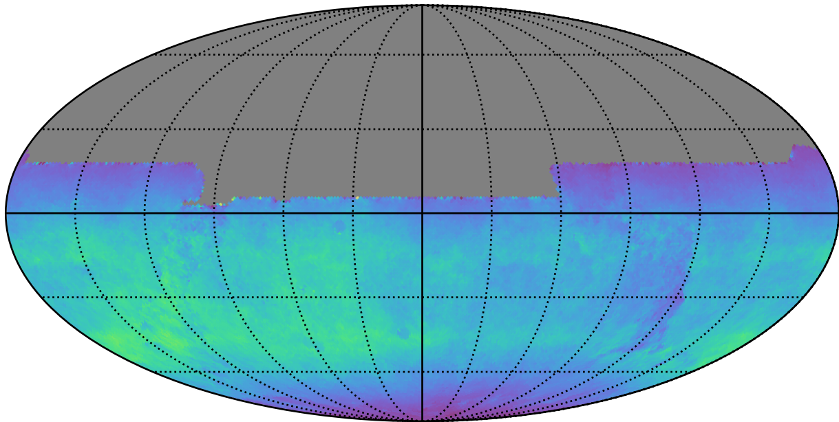
too_ignore_10_1v3.4_10yrs All sky y band: Normalized Teff
