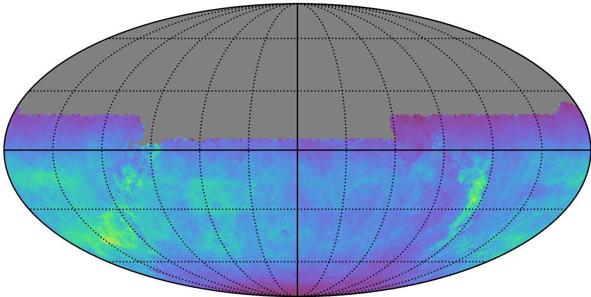
too_ignore_10_1v3.4_10yrs All sky u band: Normalized Teff
