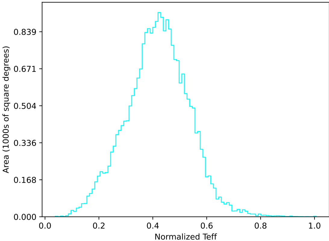
too_ignore_10_1v3.4_10yrs All sky u band: Normalized Teff
