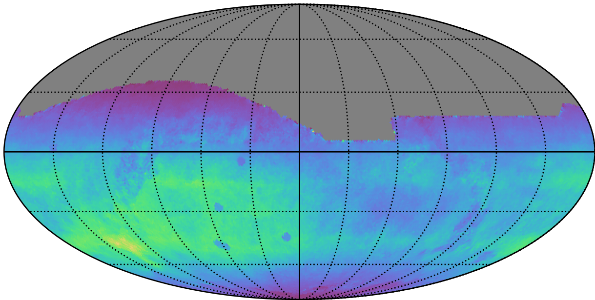
too_ignore_10_1v3.4_10yrs All sky r band: Normalized Teff
