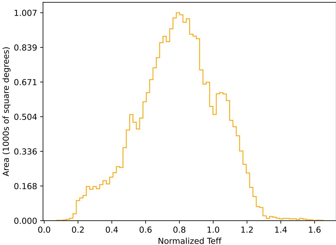
too_ignore_10_1v3.4_10yrs All sky r band: Normalized Teff
