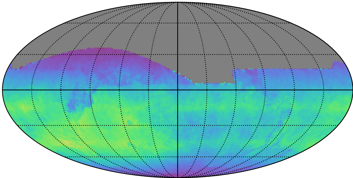
too_ignore_10_1v3.4_10yrs All sky i band: Normalized Teff
