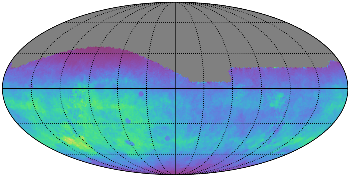
too_ignore_10_1v3.4_10yrs All sky g band: Normalized Teff
