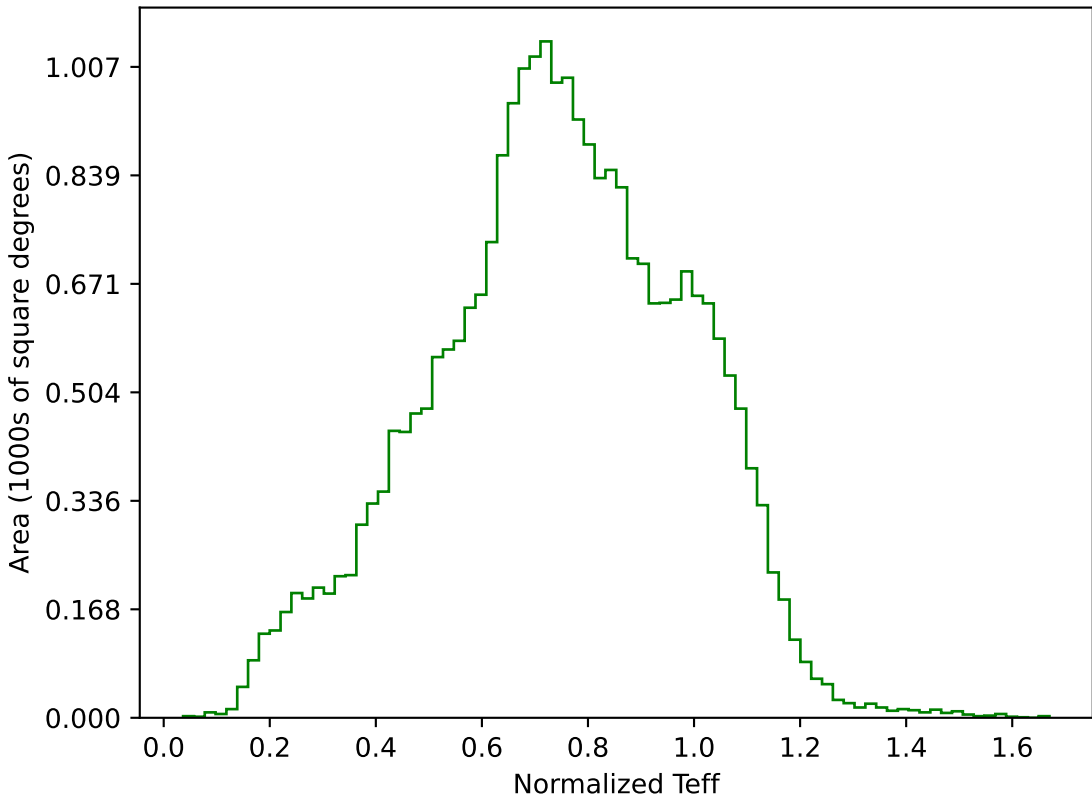
too_ignore_10_1v3.4_10yrs All sky g band: Normalized Teff
