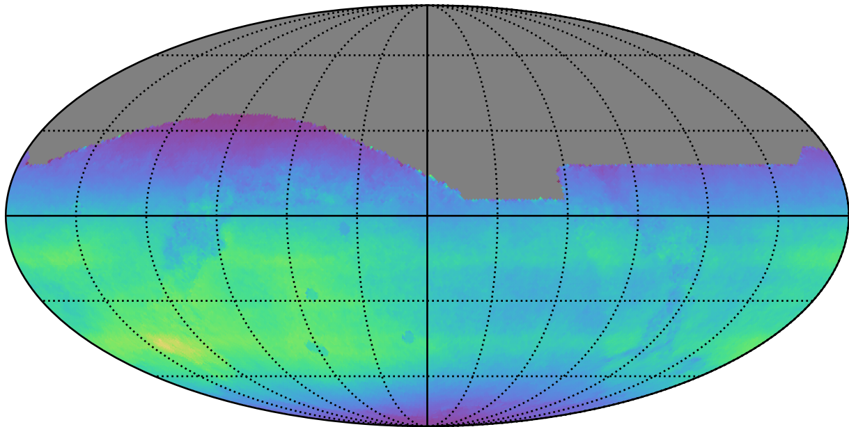
too_ignore_10_1v3.4_10yrs All sky all bands: Normalized Teff
