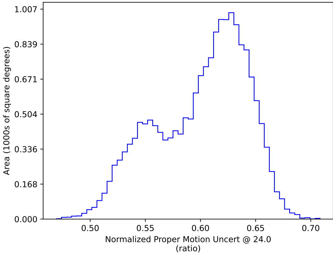
too_ignore_10_1v3.4_10yrs WFD: Normalized Proper Motion Uncert @ 24.0
