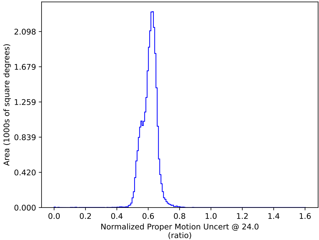
too_ignore_10_1v3.4_10yrs All sky: Normalized Proper Motion Uncert @ 24.0
