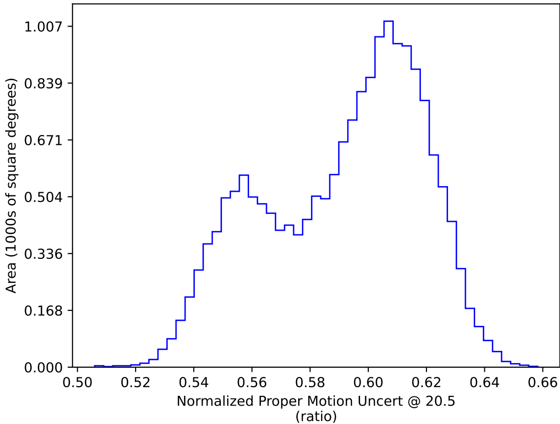
too_ignore_10_1v3.4_10yrs WFD: Normalized Proper Motion Uncert @ 20.5
