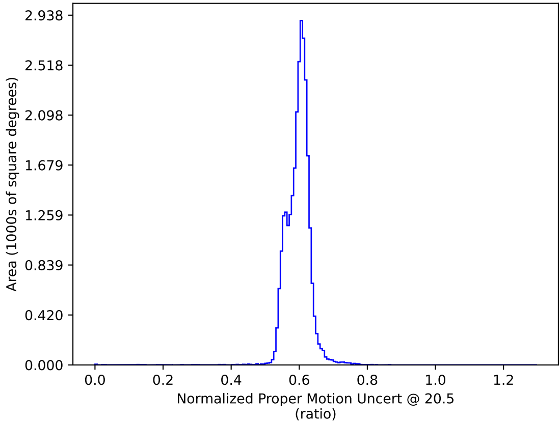
too_ignore_10_1v3.4_10yrs All sky: Normalized Proper Motion Uncert @ 20.5
