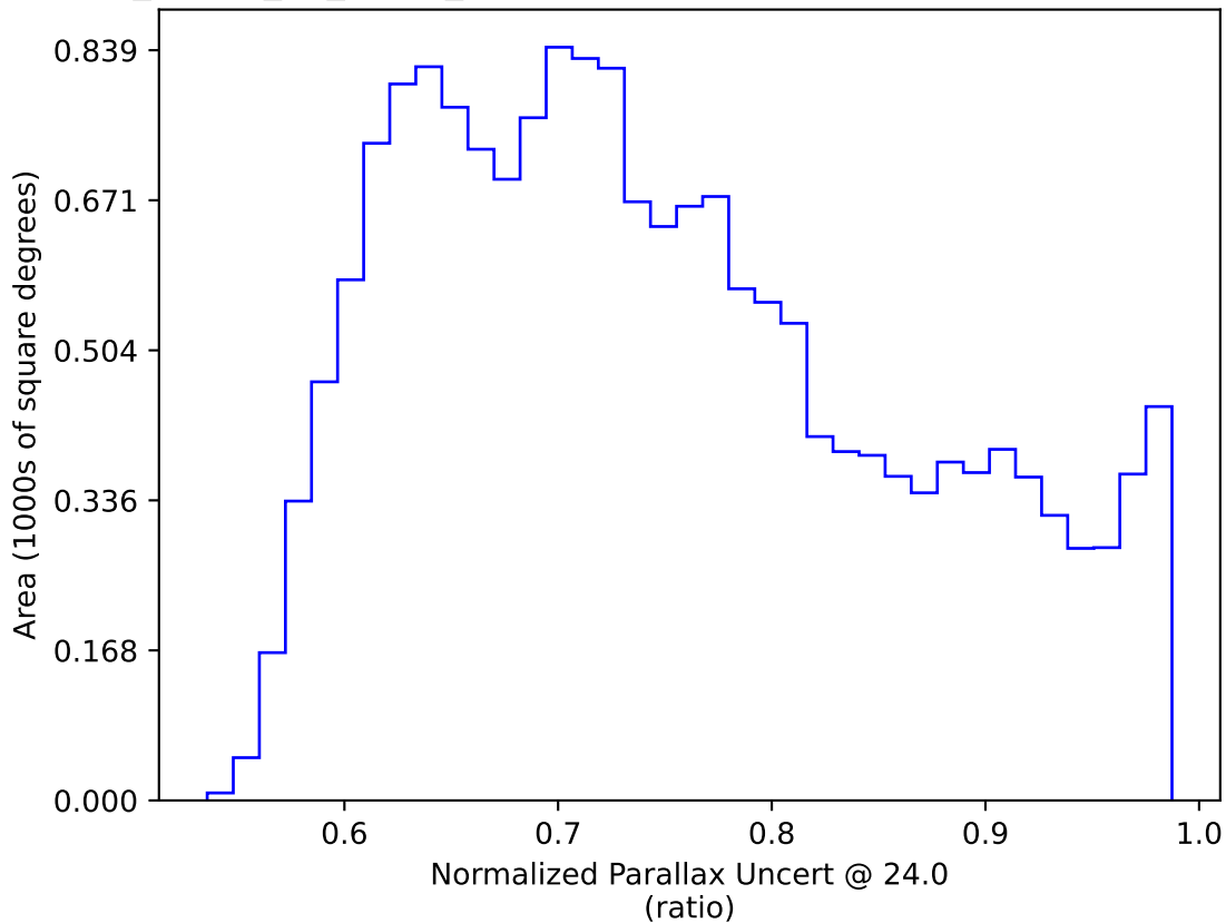
too_ignore_10_1v3.4_10yrs WFD: Normalized Parallax Uncert @ 24.0
