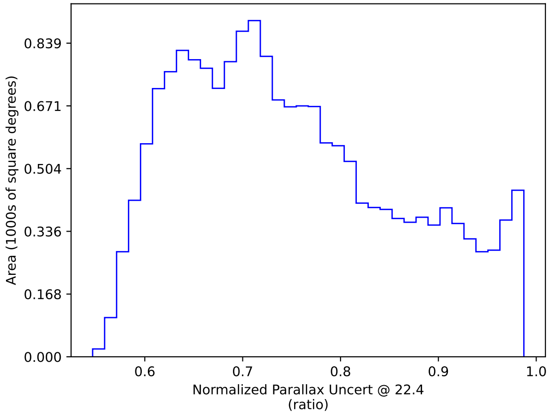
too_ignore_10_1v3.4_10yrs WFD: Normalized Parallax Uncert @ 22.4
