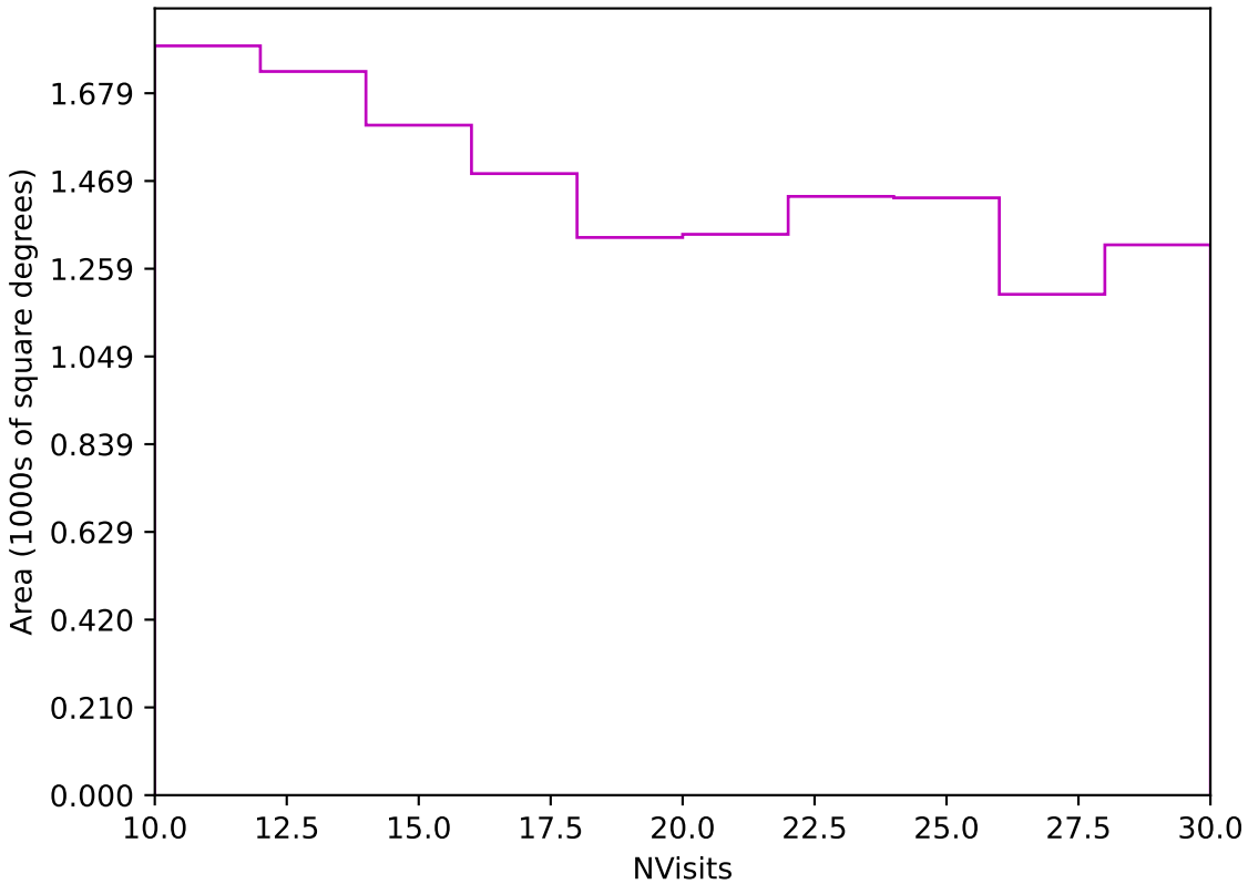
too_ignore_10_1v3.4_10yrs Yr 3-4 z band: NVisits
