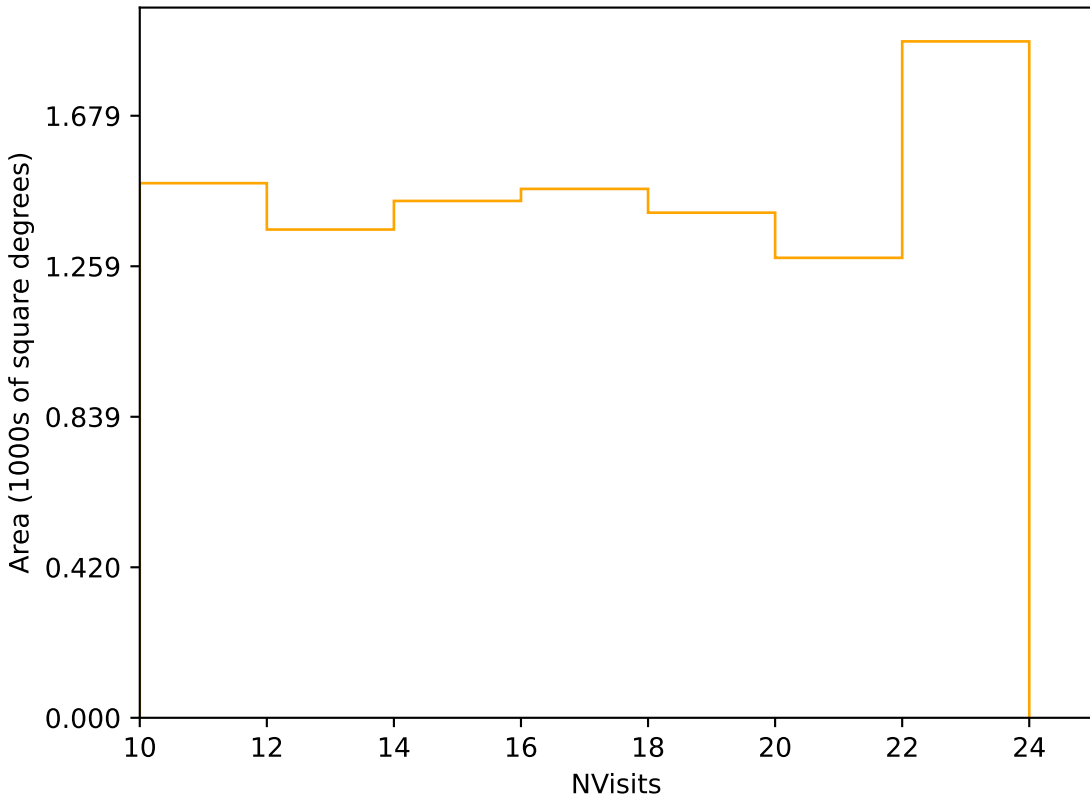
too_ignore_10_1v3.4_10yrs Yr 3-4 r band: NVisits
