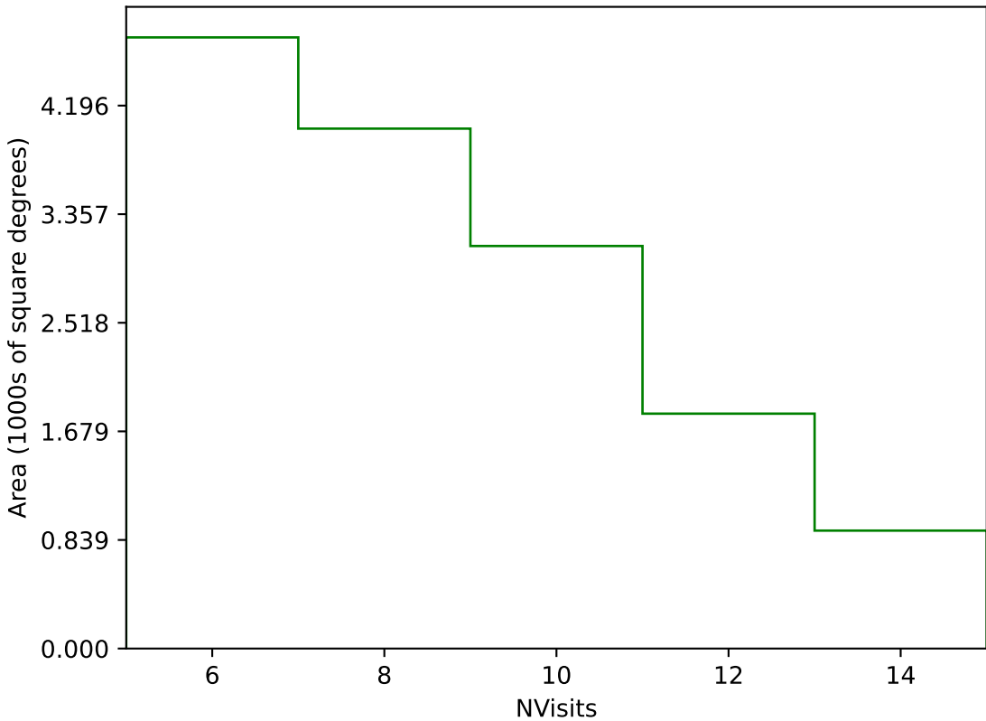
too_ignore_10_1v3.4_10yrs Yr 3-4 g band: NVisits
