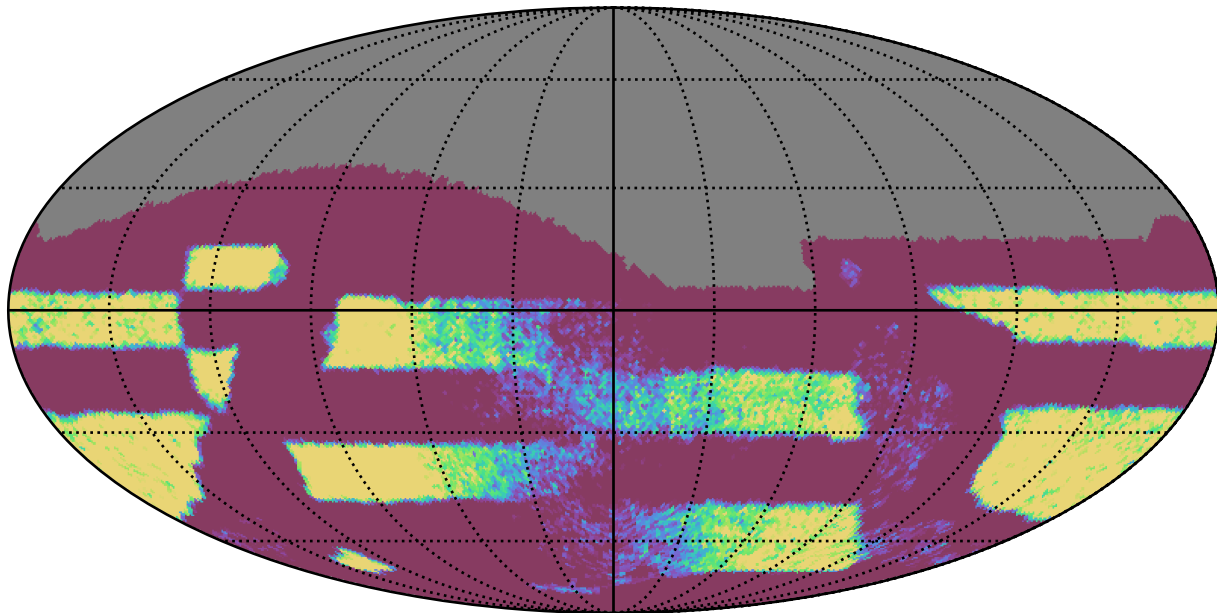
too_ignore_10_1v3.4_10yrs Yr 3-4 all bands: NVisits
