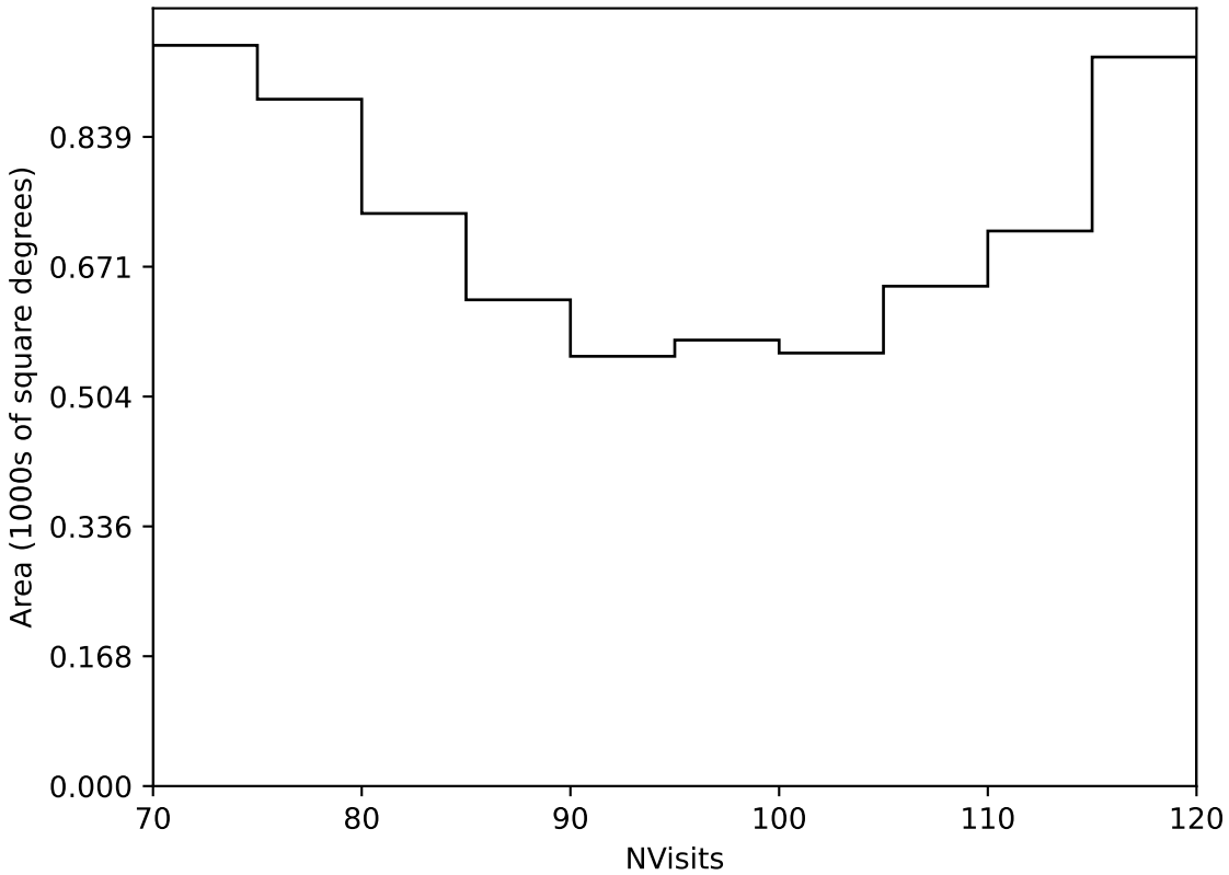
too_ignore_10_1v3.4_10yrs Yr 3-4 all bands: NVisits
