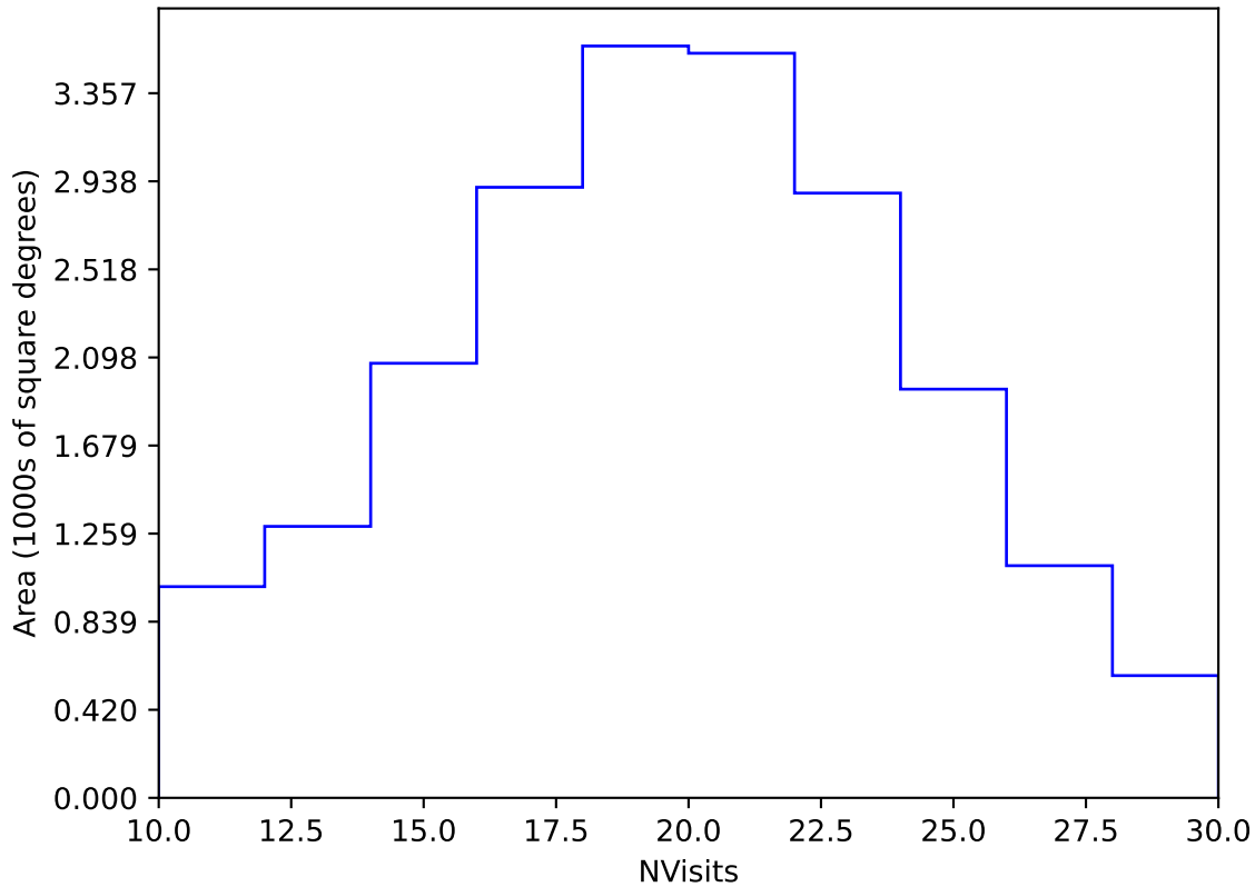
too_ignore_10_1v3.4_10yrs Yr 1 y band: NVisits
