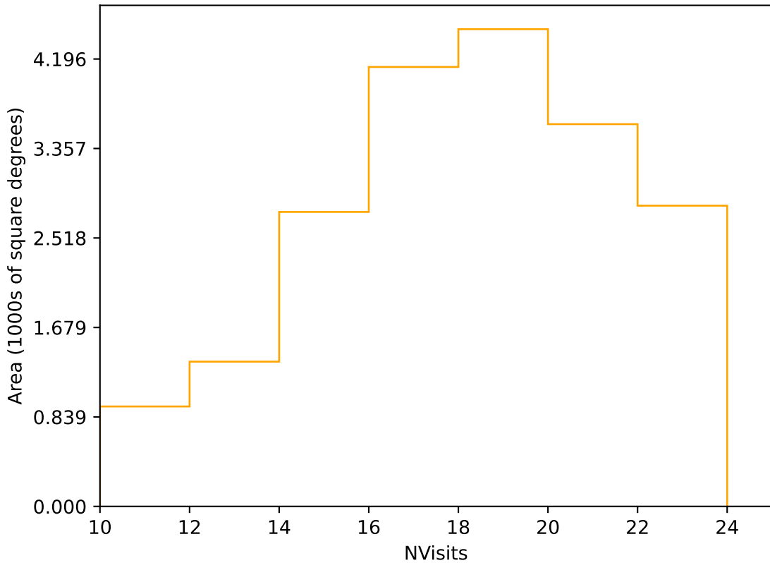
too_ignore_10_1v3.4_10yrs Yr 1 r band: NVisits
