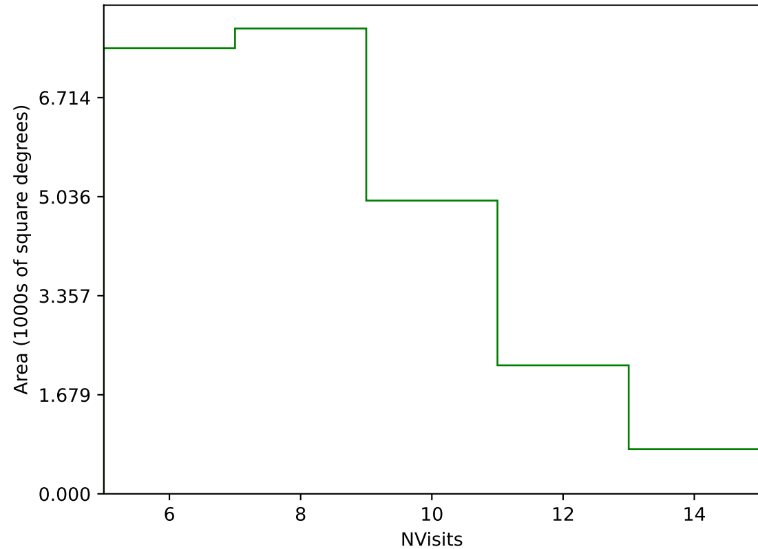
too_ignore_10_1v3.4_10yrs Yr 1 g band: NVisits
