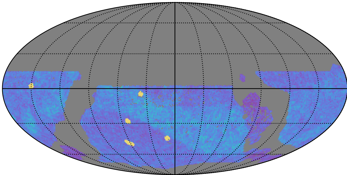
too_ignore_10_1v3.4_10yrs WFD z band: NVisits
