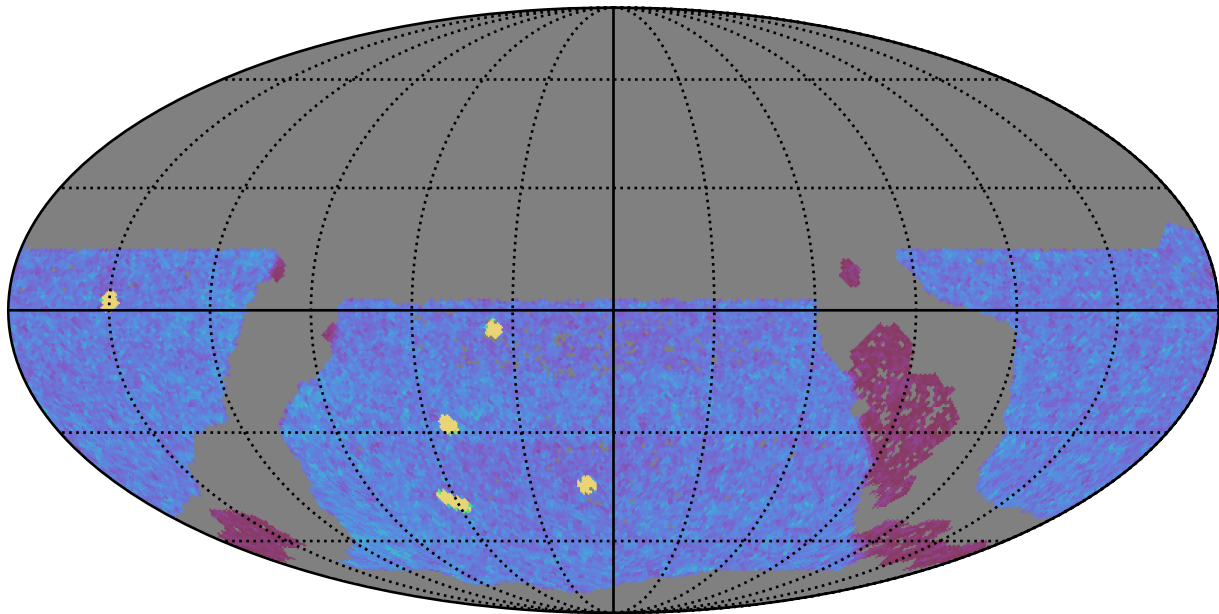
too_ignore_10_1v3.4_10yrs WFD y band: NVisits
