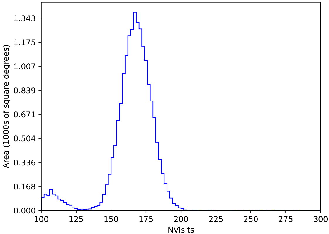
too_ignore_10_1v3.4_10yrs WFD y band: NVisits
