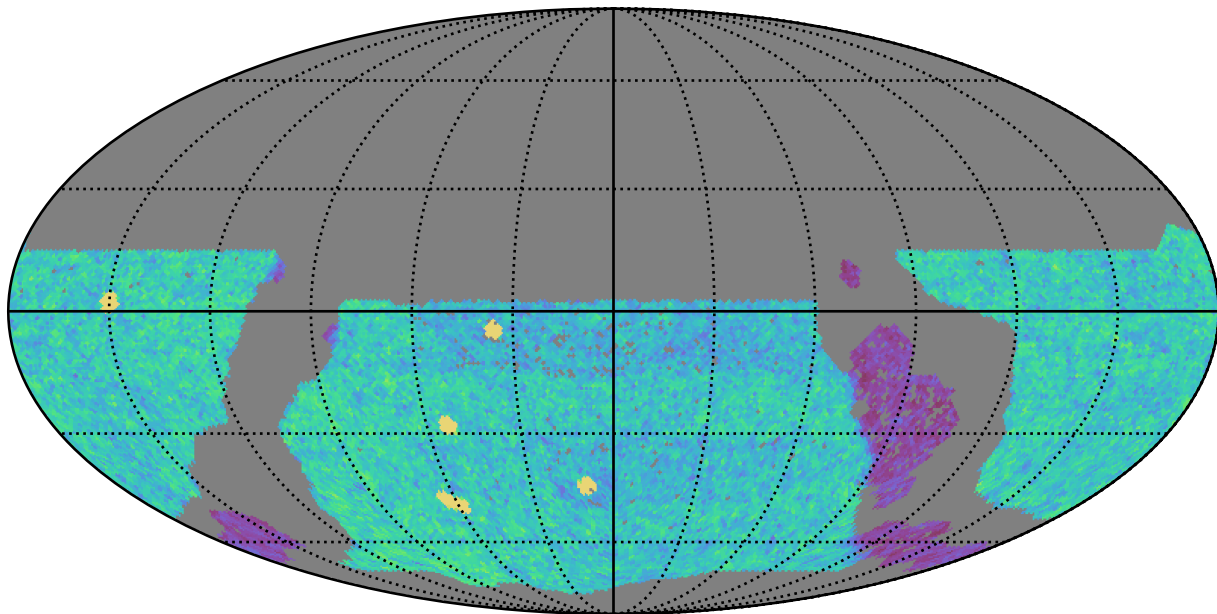
too_ignore_10_1v3.4_10yrs WFD u band: NVisits
