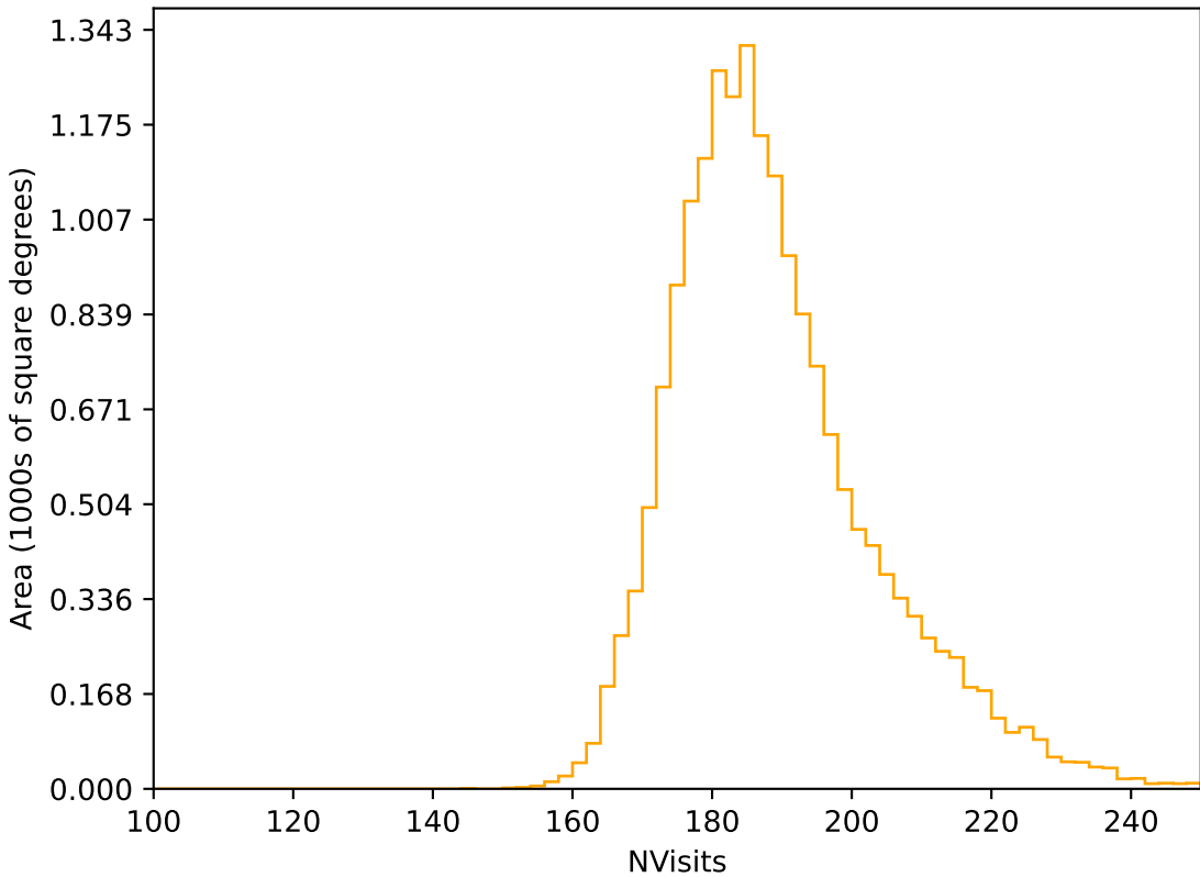
too_ignore_10_1v3.4_10yrs WFD r band: NVisits
