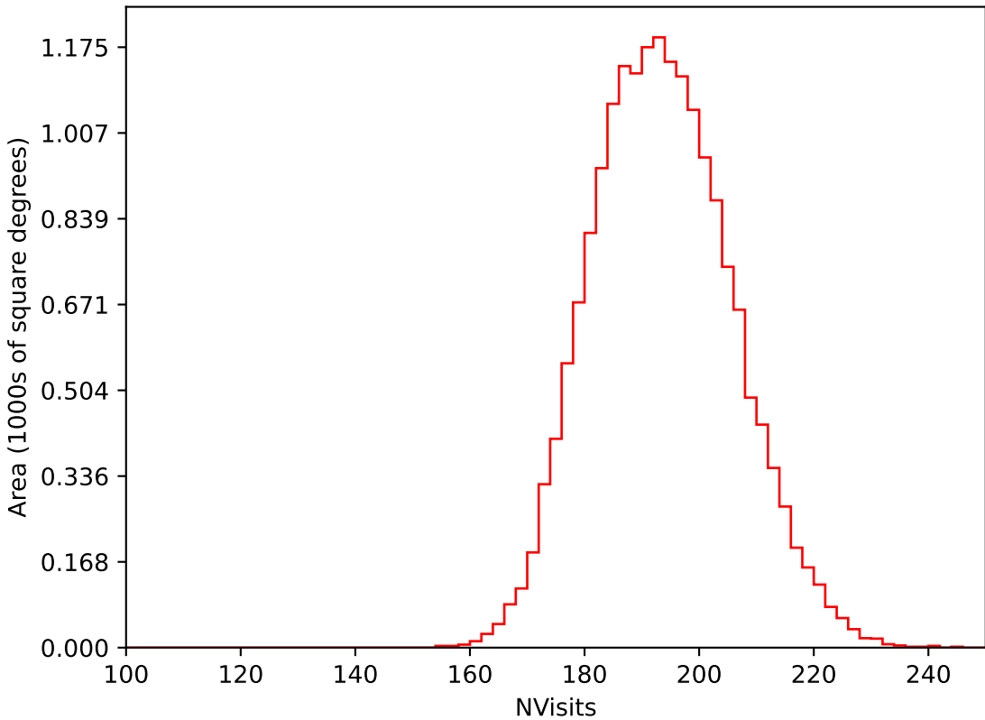
too_ignore_10_1v3.4_10yrs WFD i band: NVisits
