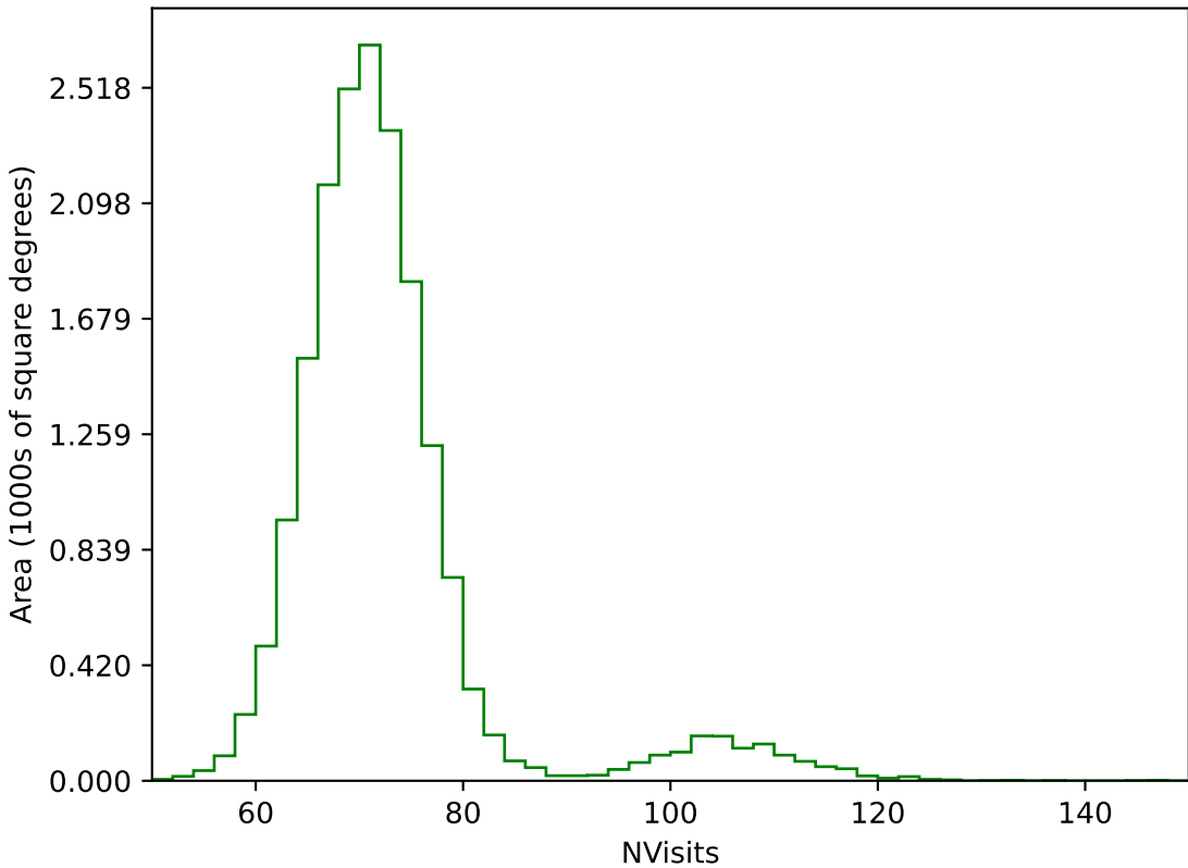
too_ignore_10_1v3.4_10yrs WFD g band: NVisits
