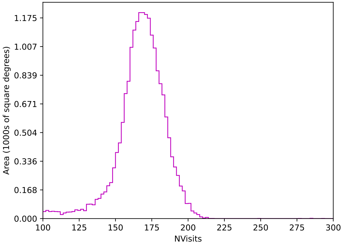
too_ignore_10_1v3.4_10yrs All sky z band: NVisits
