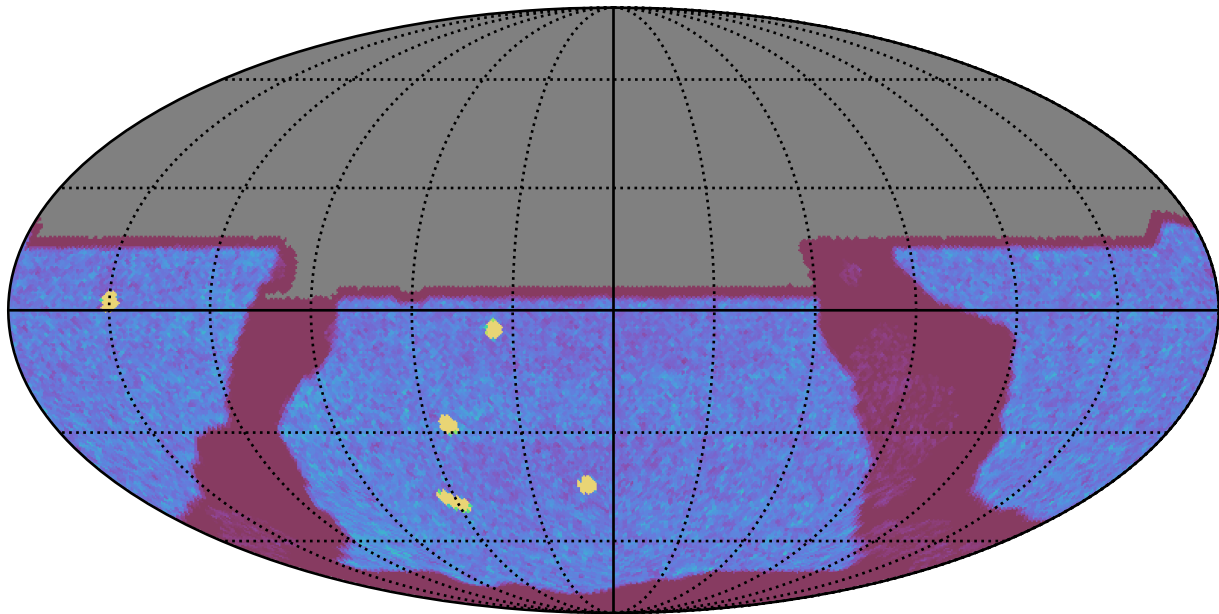
too_ignore_10_1v3.4_10yrs All sky y band: NVisits
