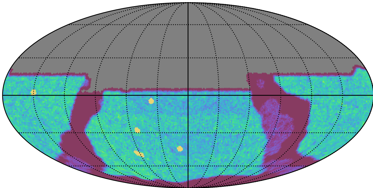
too_ignore_10_1v3.4_10yrs All sky u band: NVisits
