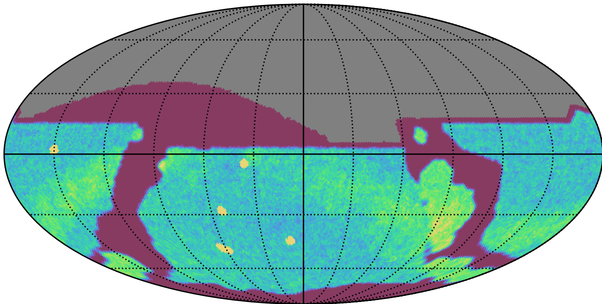
too_ignore_10_1v3.4_10yrs All sky r band: NVisits
