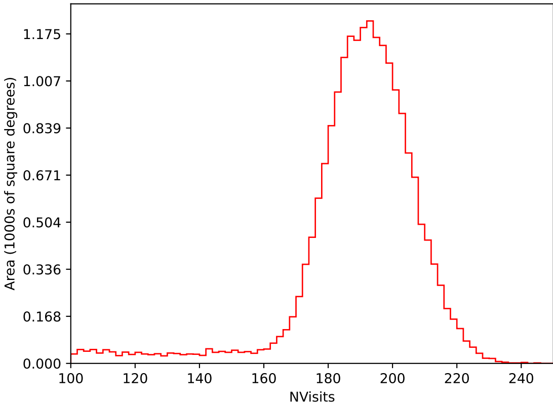
too_ignore_10_1v3.4_10yrs All sky i band: NVisits
