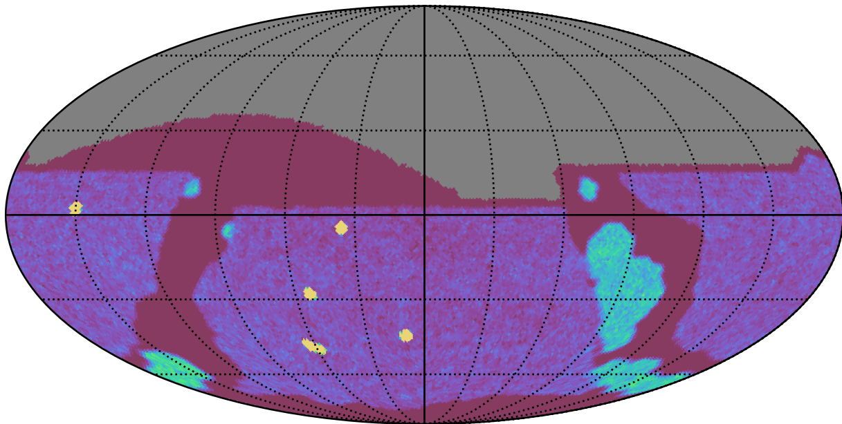
too_ignore_10_1v3.4_10yrs All sky g band: NVisits
