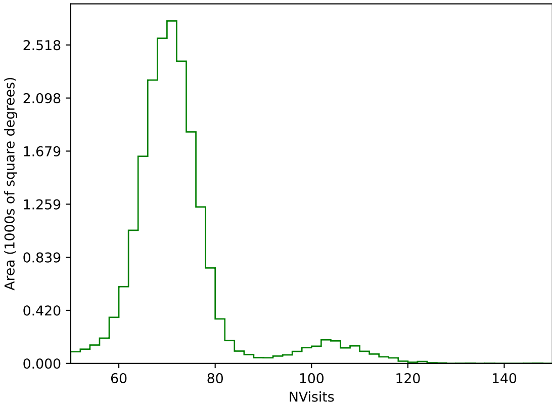
too_ignore_10_1v3.4_10yrs All sky g band: NVisits
