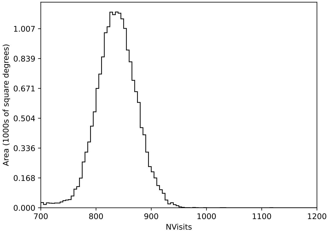
too_ignore_10_1v3.4_10yrs All sky all bands: NVisits
