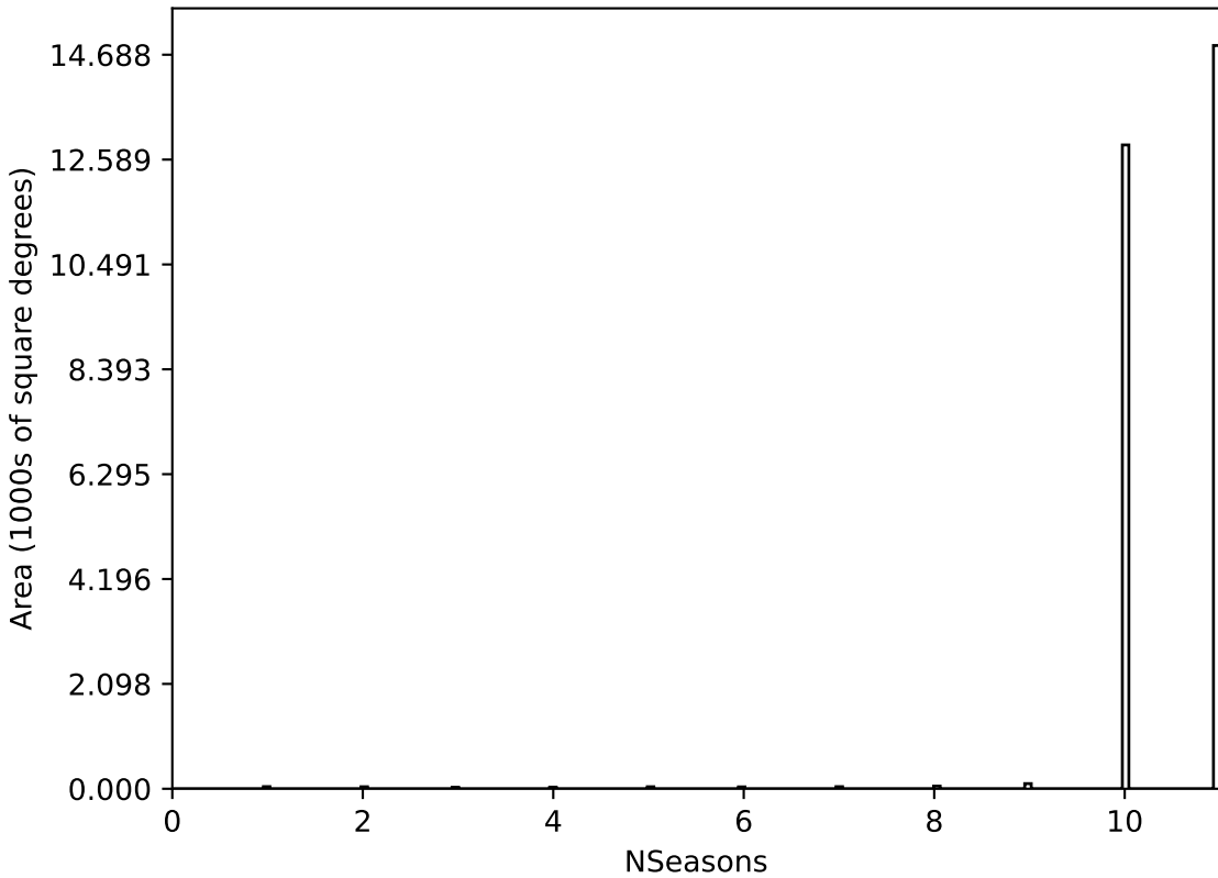
too_ignore_10_1v3.4_10yrs All sky all bands: NSeasons
