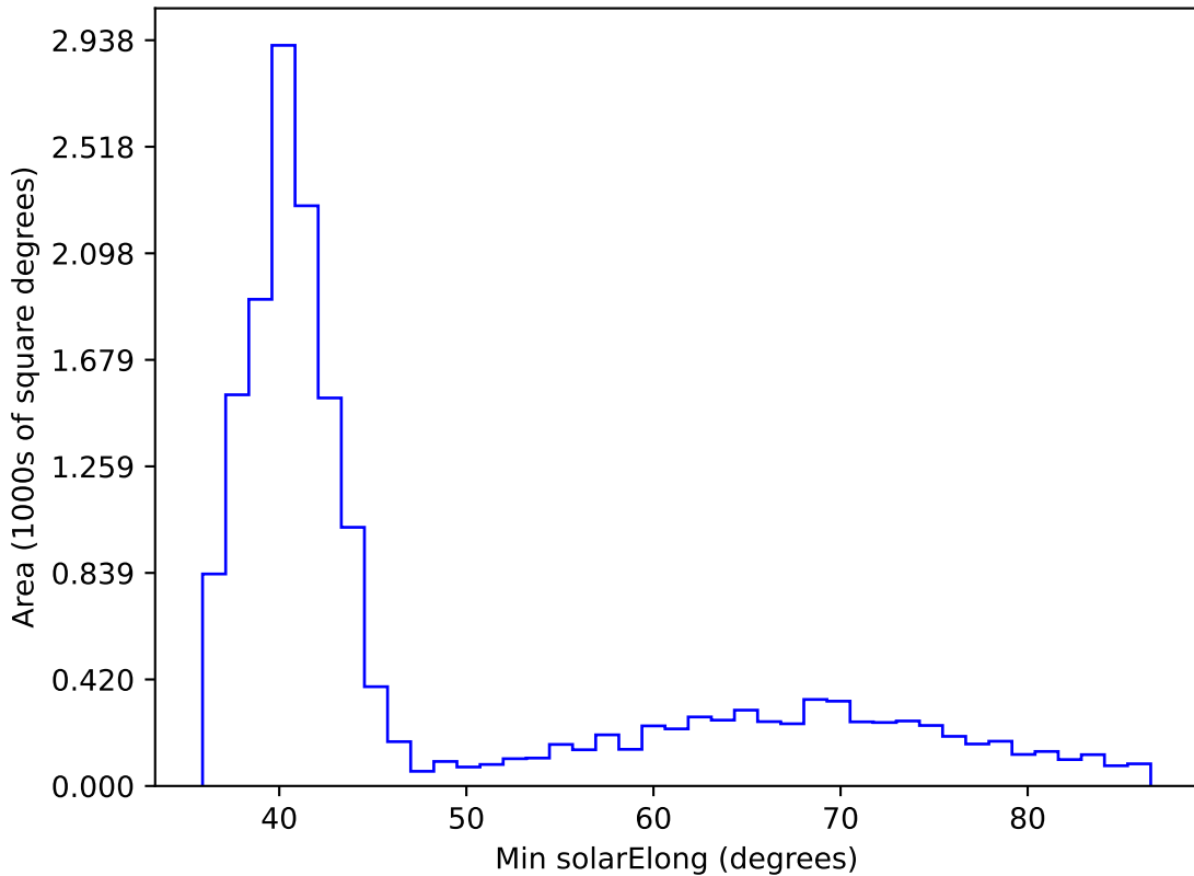
too_ignore_10_1v3.4_10yrs WFD z band: Min solarElong
