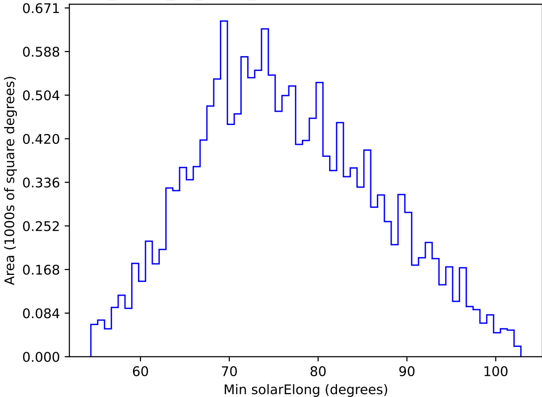
too_ignore_10_1v3.4_10yrs WFD u band: Min solarElong
