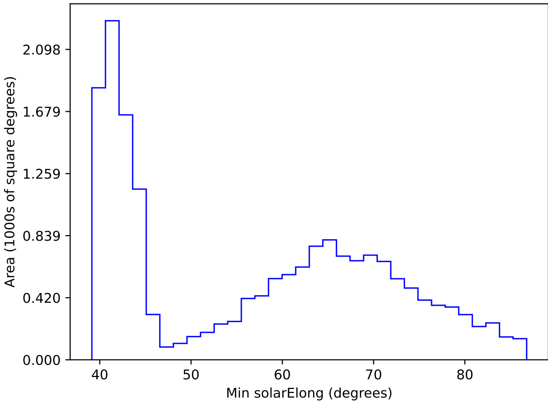
too_ignore_10_1v3.4_10yrs WFD r band: Min solarElong
