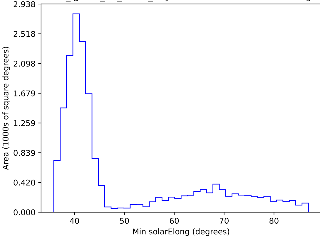
too_ignore_10_1v3.4_10yrs WFD i band: Min solarElong
